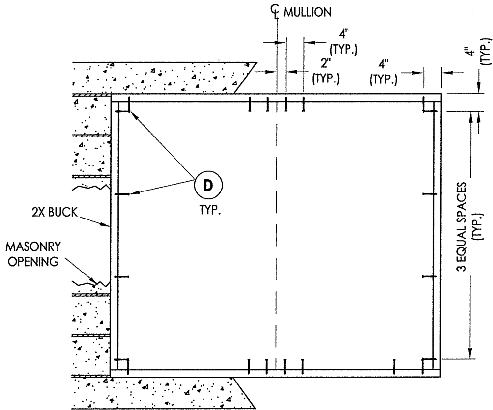
BUCK ANCHORING
