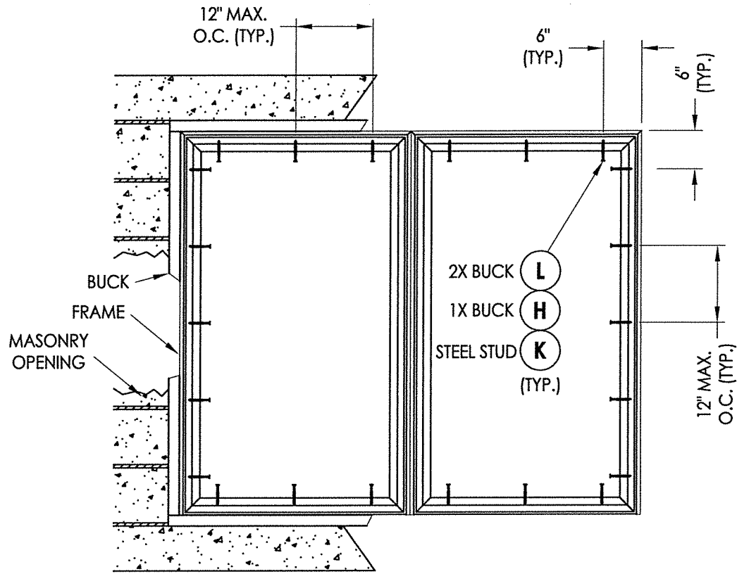
FRAME ANCHORING
